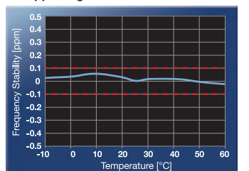
\pm 0.1 ppm High Precision TCXO
